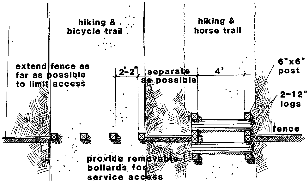
gate plan
