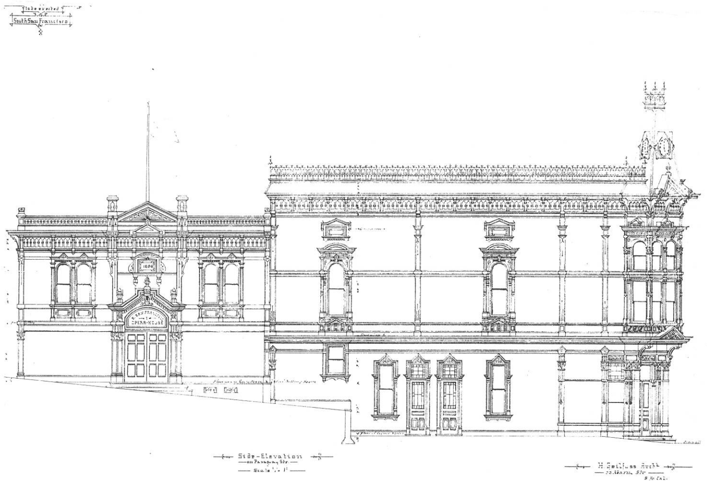
SOUTH SAN FRANCISCO OPERA HOUSE San Francisco, CA From the collection of San Francisco Architectural Heritage Date: circa 1888 Exterior – Architectural drawing, South San Francisco Opera House and Masonic Hall, Henry Geilfuss; looking south Figure 1 of 12
