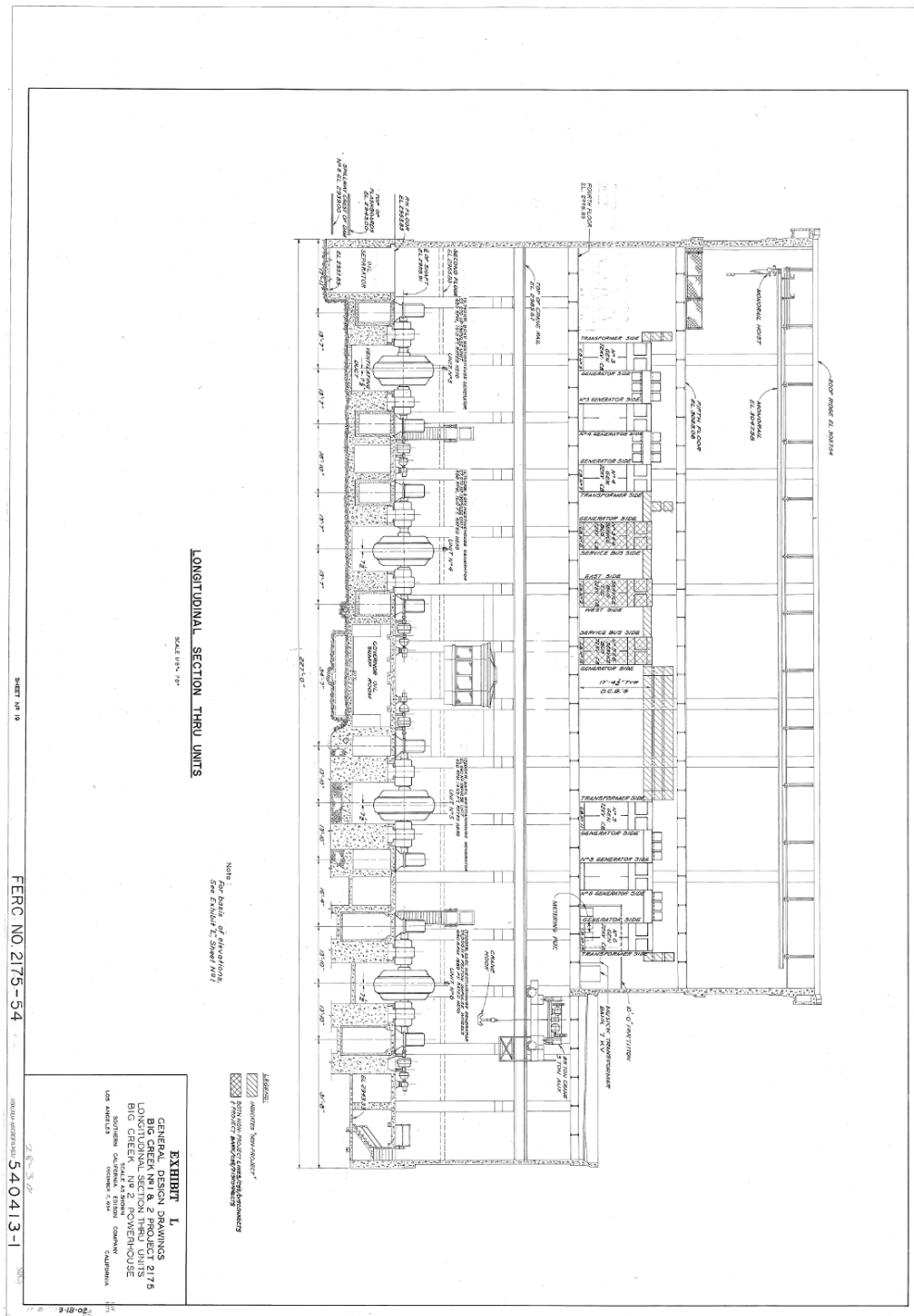
Figure 26: Powerhouse No. 2 General Design Drawing, 1954. Drawing No. 540413-1. On file at SCE Northern Hydro Headquarters.
