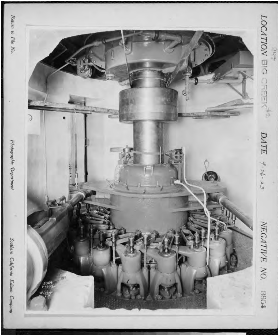
Figure 52: Powerhouse No. 3 close-up of turbine, 1923. Image No. SCE-02-08854, Huntington Digital Library.
